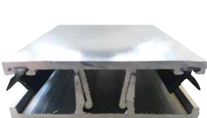
Aluminium Joiner showing Butterfly rubber for inside joiners
